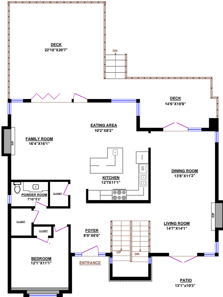
MAIN FLOOR
